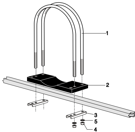
Montagevariante I
