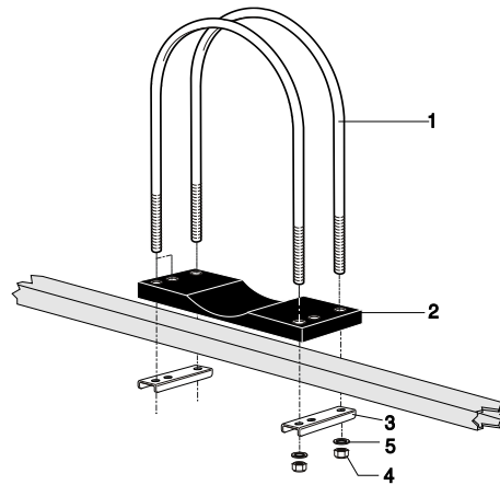
Montagevariante II
